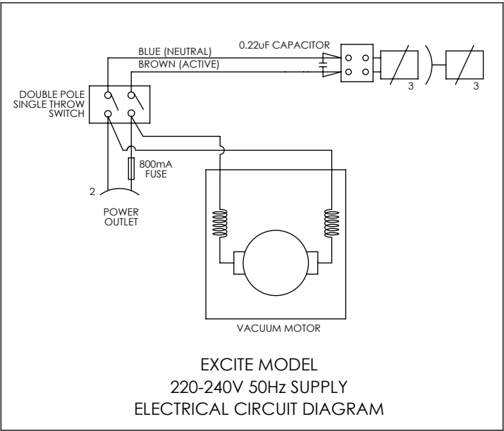
15721200 EXCITE ASSEMBLY
